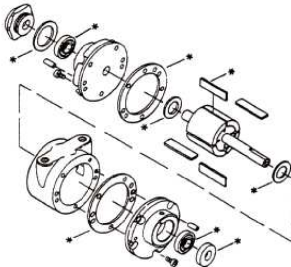
AIR MOTOR 000.740.002 * DENOTES PART OF AIR MOTOR REBUILD KIT. (PART NUMBER 669.900.111)
