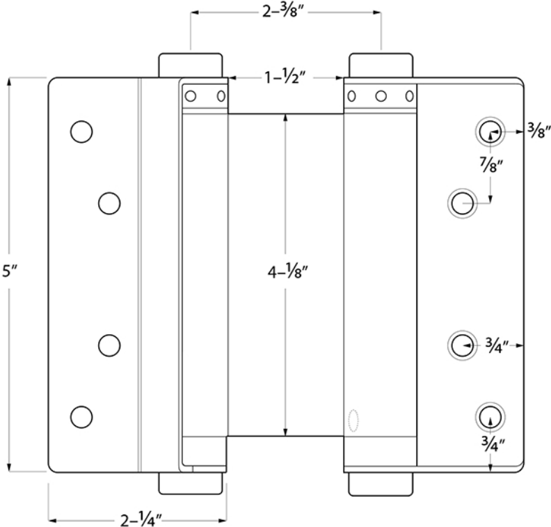
OPEN POSITION
