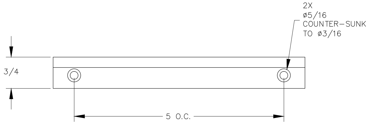
FRONT VIEW
