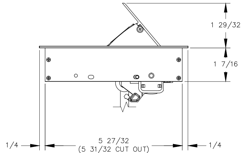
RIGHT VIEW
