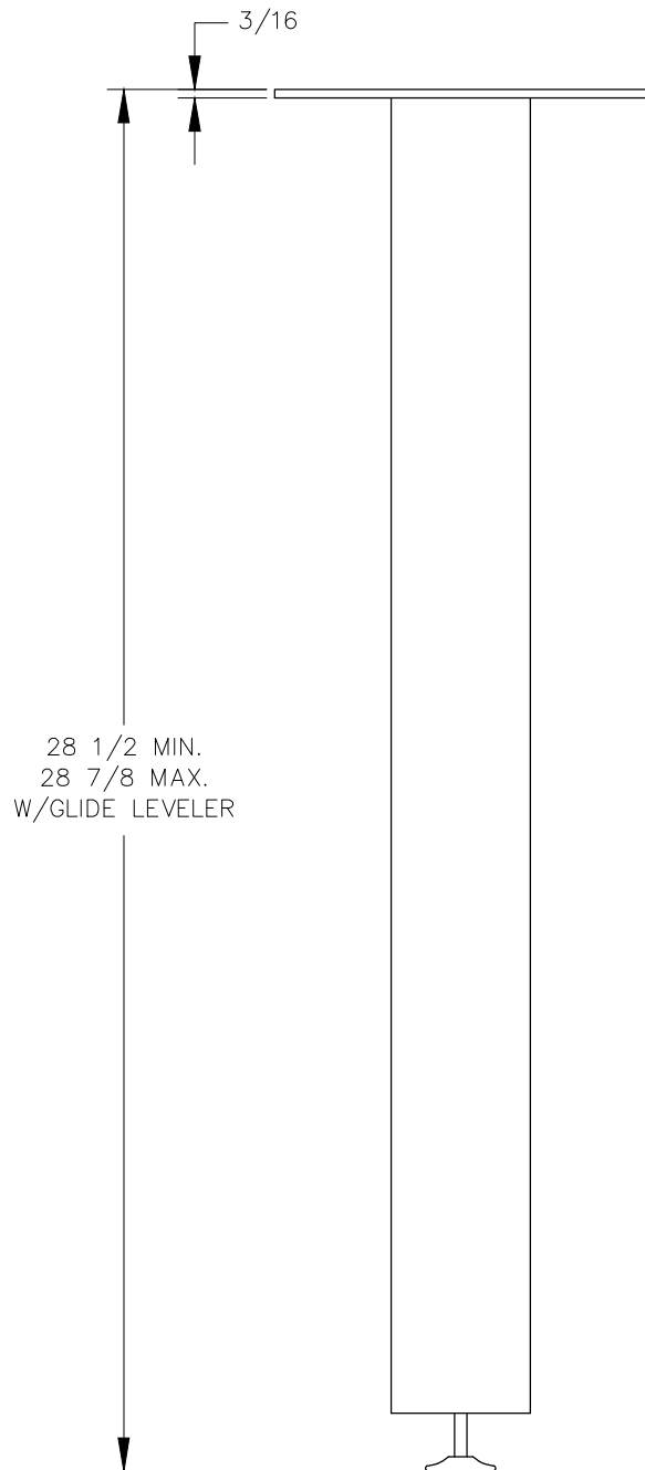
FRONT VIEW
