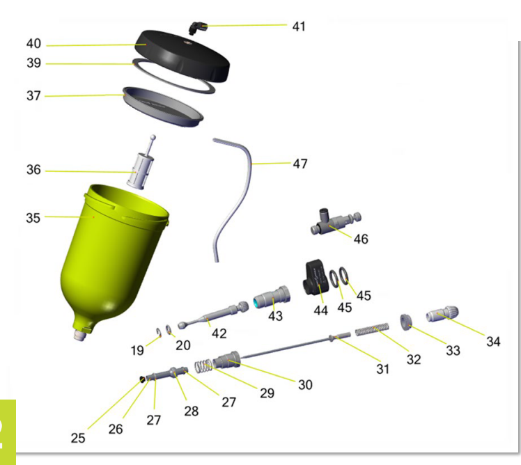
FPRO GSP - EXPLODED VIEW C2
