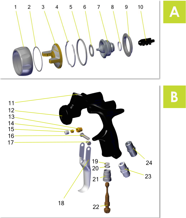
FPRO G - EXPLODED VIEW C1
