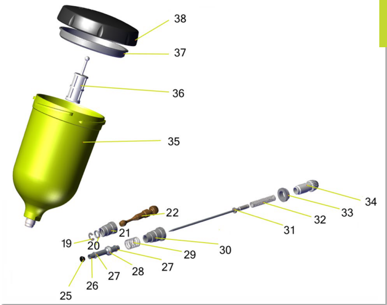
FPRO G - EXPLODED VIEW C1
