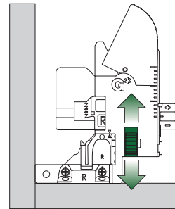
Front Locking Device
