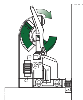
2D/3D Front Locking Devices
