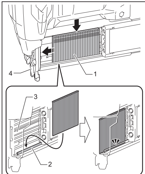
► 1. Fastener strip 2. Magazine plate 3. Magazine 4. Driver guide
