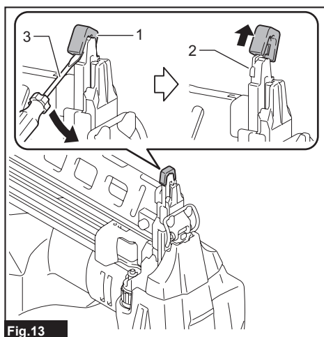
► 1. Nose adapter 2. Contact element 3. Slotted screwdriver
