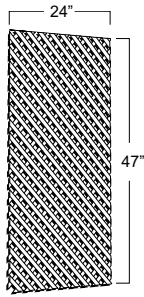
Mini Diagonal Lattice Door Insert Cell size: 1/2" Thickness: 5/32"
