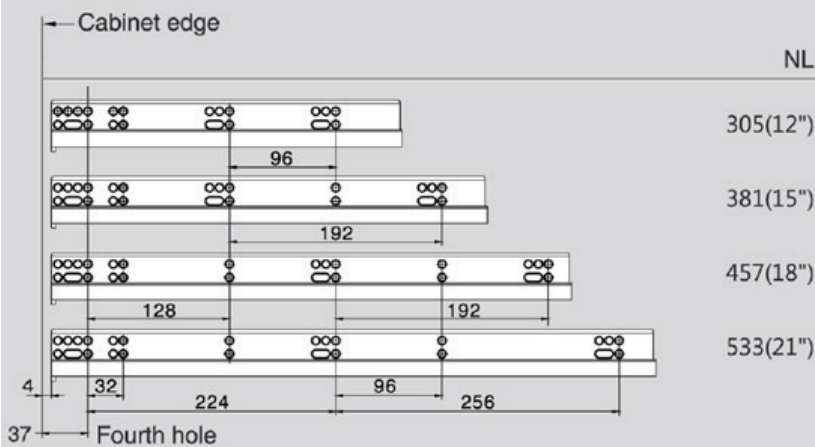
Installation Dimensions(mm)
