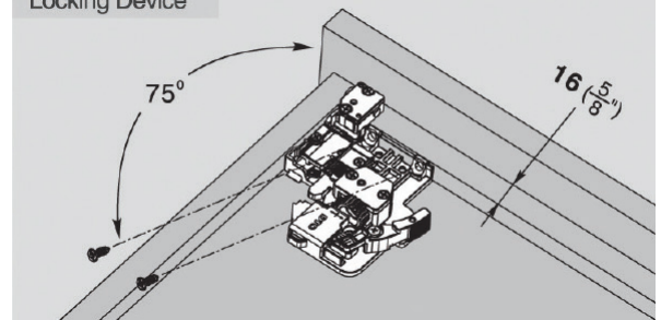
Locking Device
