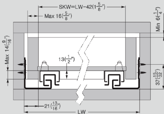
Installation Dimensions(mm)
