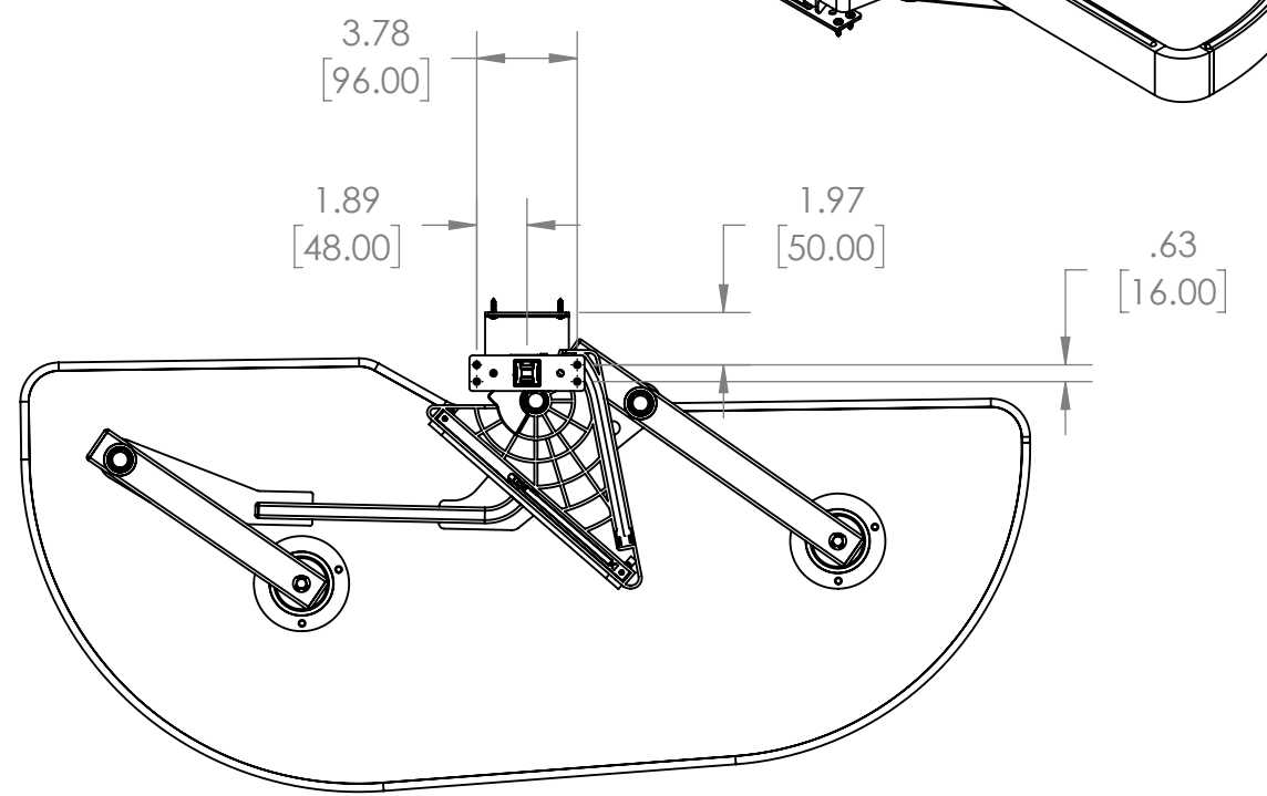
BOTTOM VIEW
