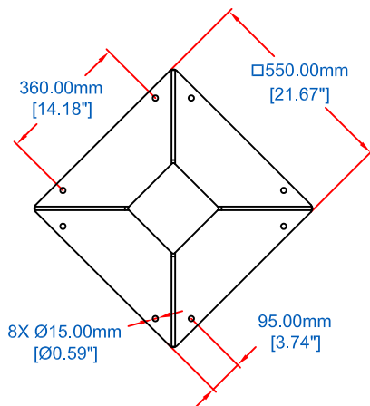
MOUNTING PATTERN SCALE 2:1
