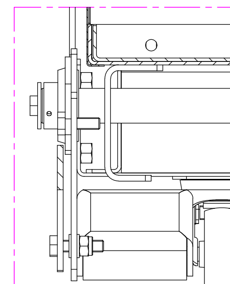
DETAIL D
